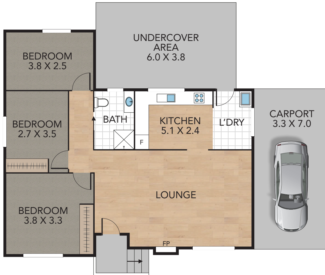
GROUND FLOOR
